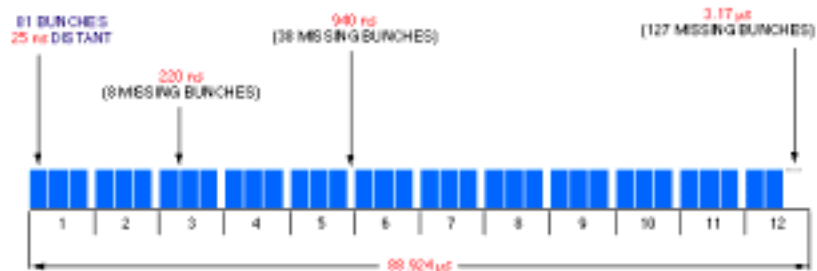
Fig. 6 Timing scheme
