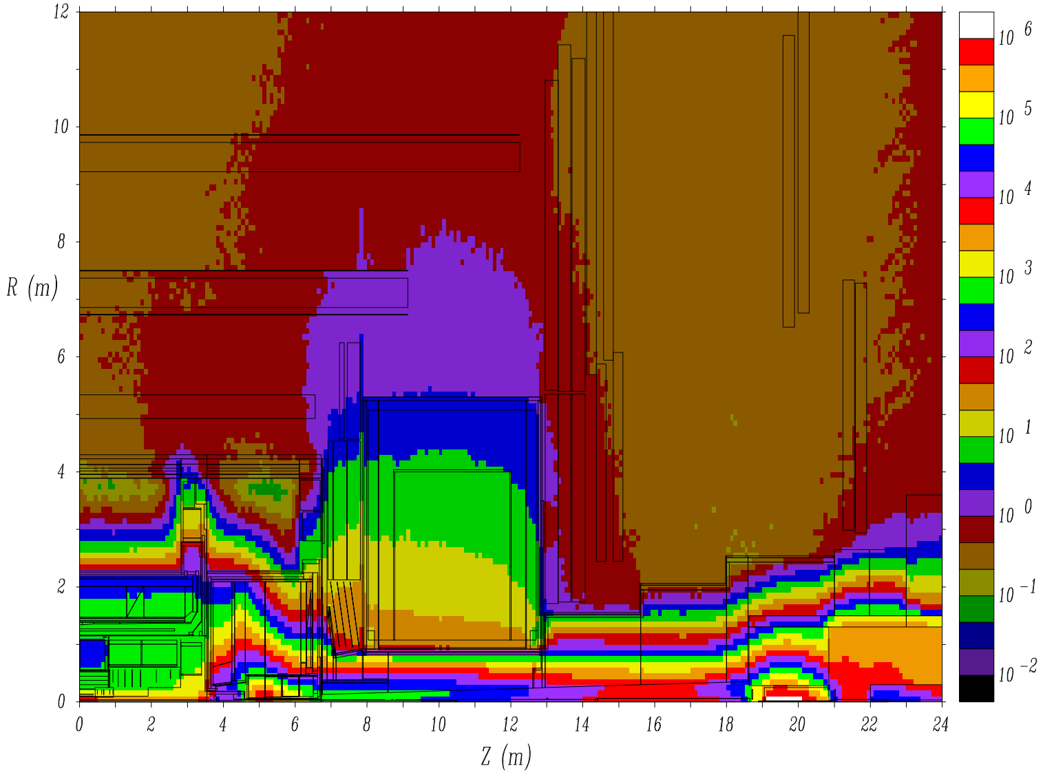
Dec01 Baseline (8220) - Neutrons > 100 keV, KHz/cm**2
