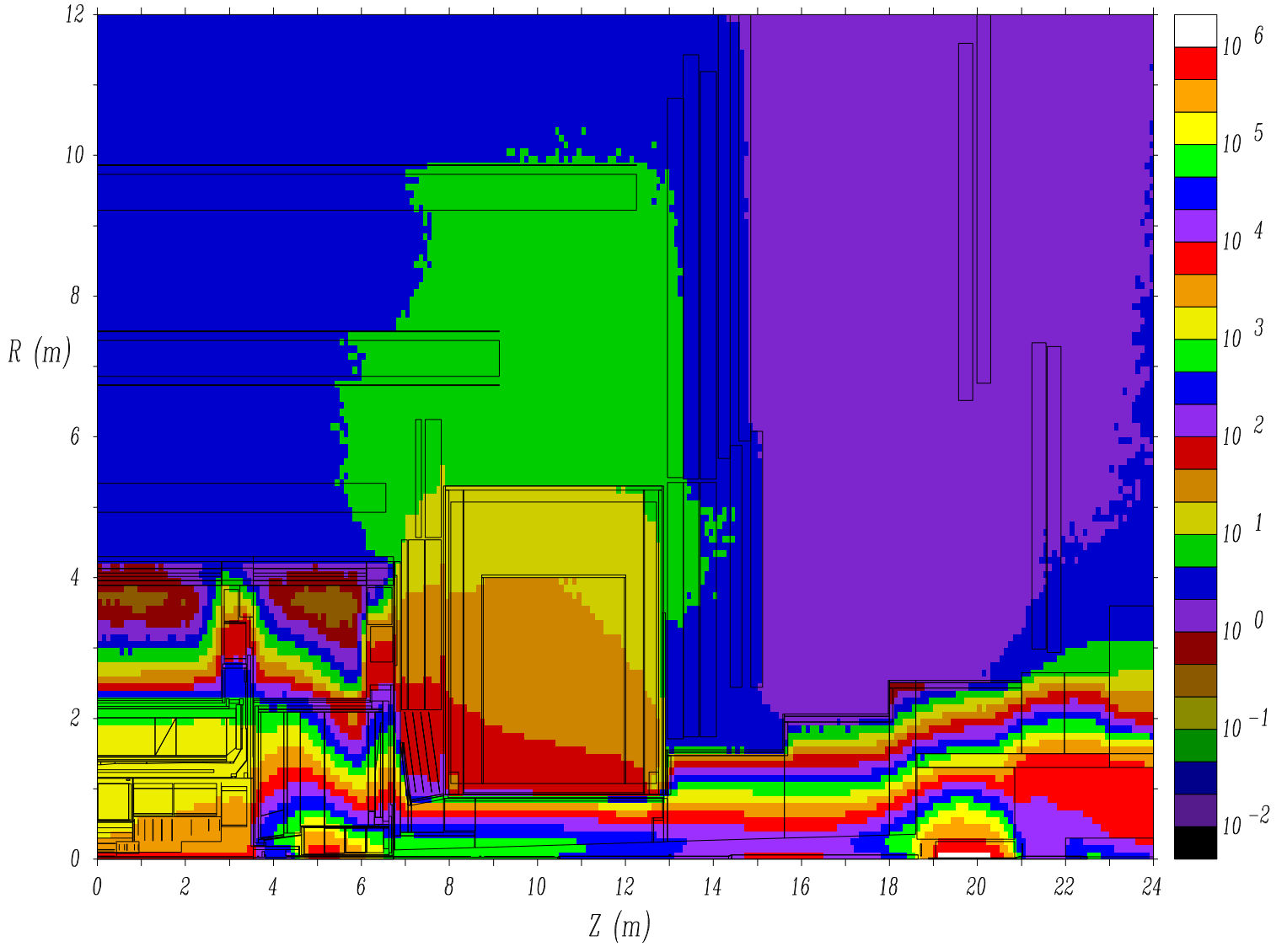
Dec01 Baseline (8220) - Neutron Flux, \text{KHz}/\text{cm}^{**2}
