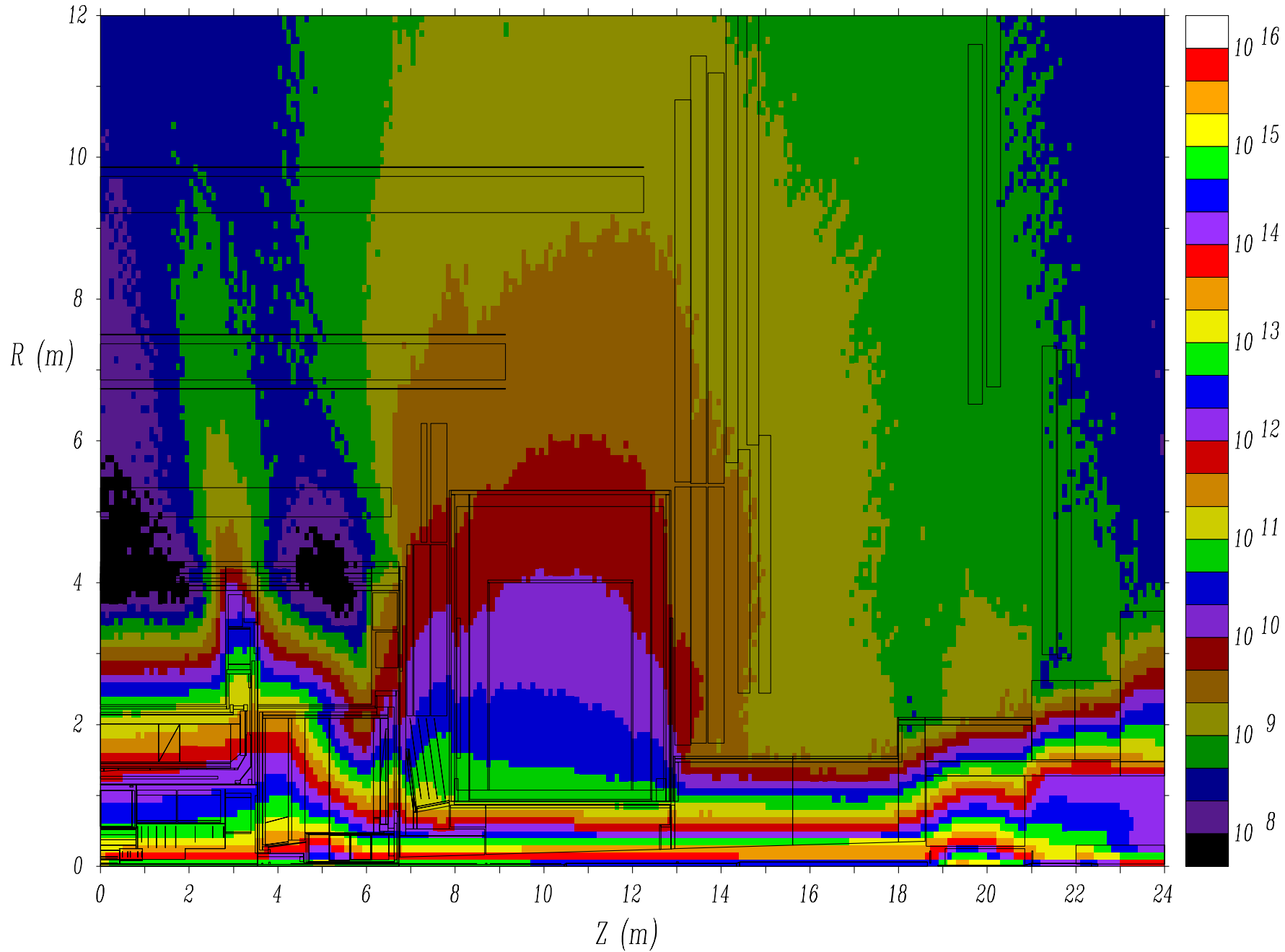
Jan03 Base (24620) - Hadron Flux > 20 MeV/cm**2/Yr
