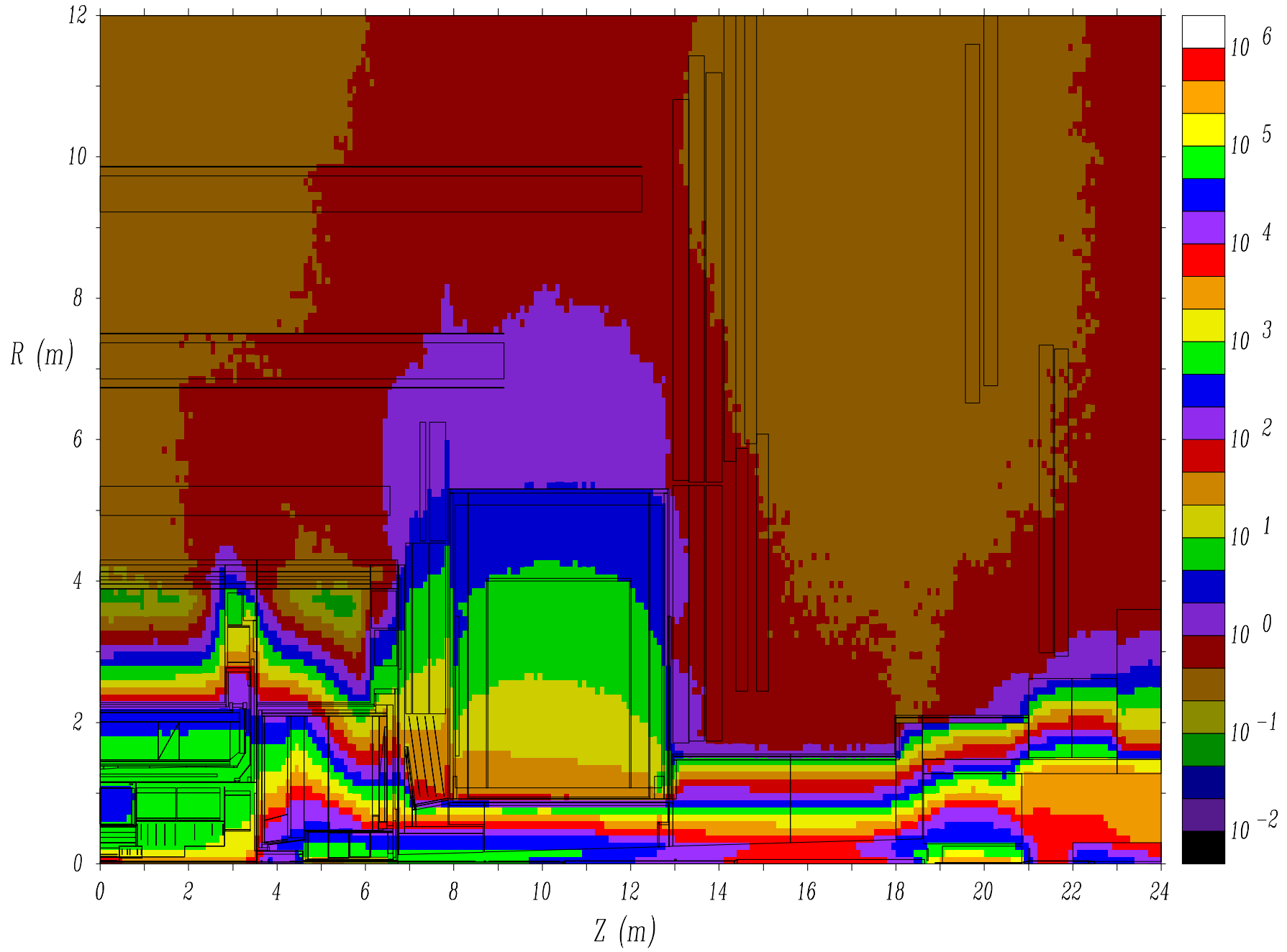
Jan03 Base (24620) - Neutrons > 100 keV, KHz/cm**2
