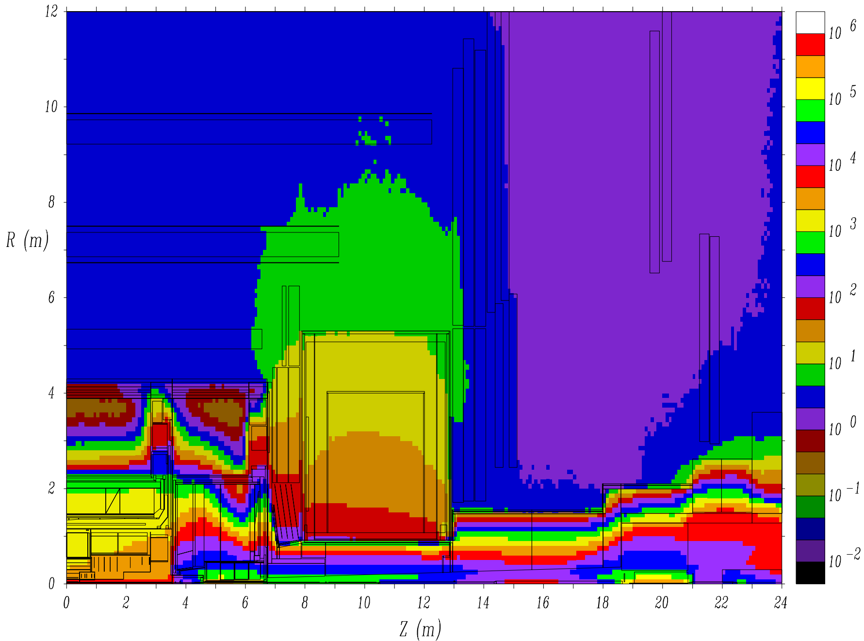
Jan03 Base (24620) - Neutron Flux, KHz/cm**2
