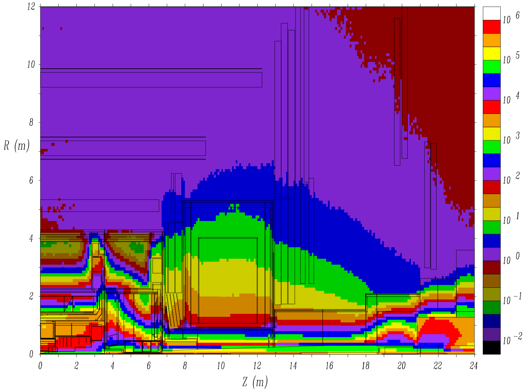
Jan03 Base (24620) - Photon Flux, KHz/cm**2
