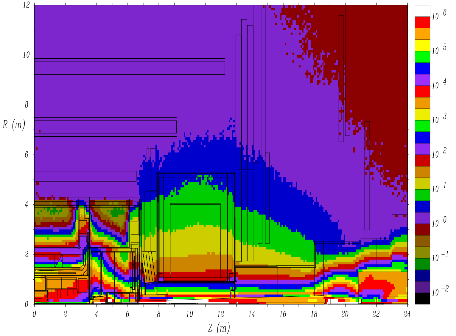
Dec01 NoJFOct1 (5920) - Photon Flux, \text{KHz}/\text{cm}^{**2}
