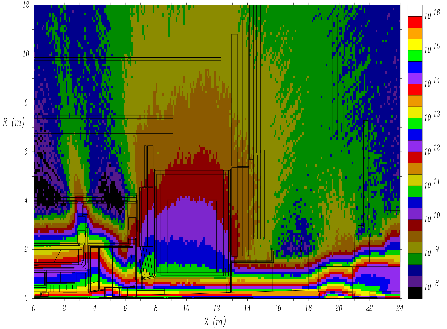
Dec01 JF0ctSameRo (5152) - Hadron Flux > 20 MeV/cm**2/Yr
