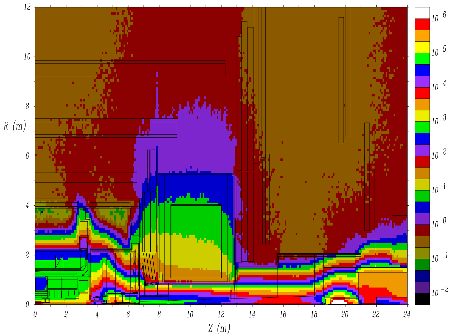
Dec01 JF0ctSameRo (5152) - Neutrons > 100 keV, KHz/cm**2
