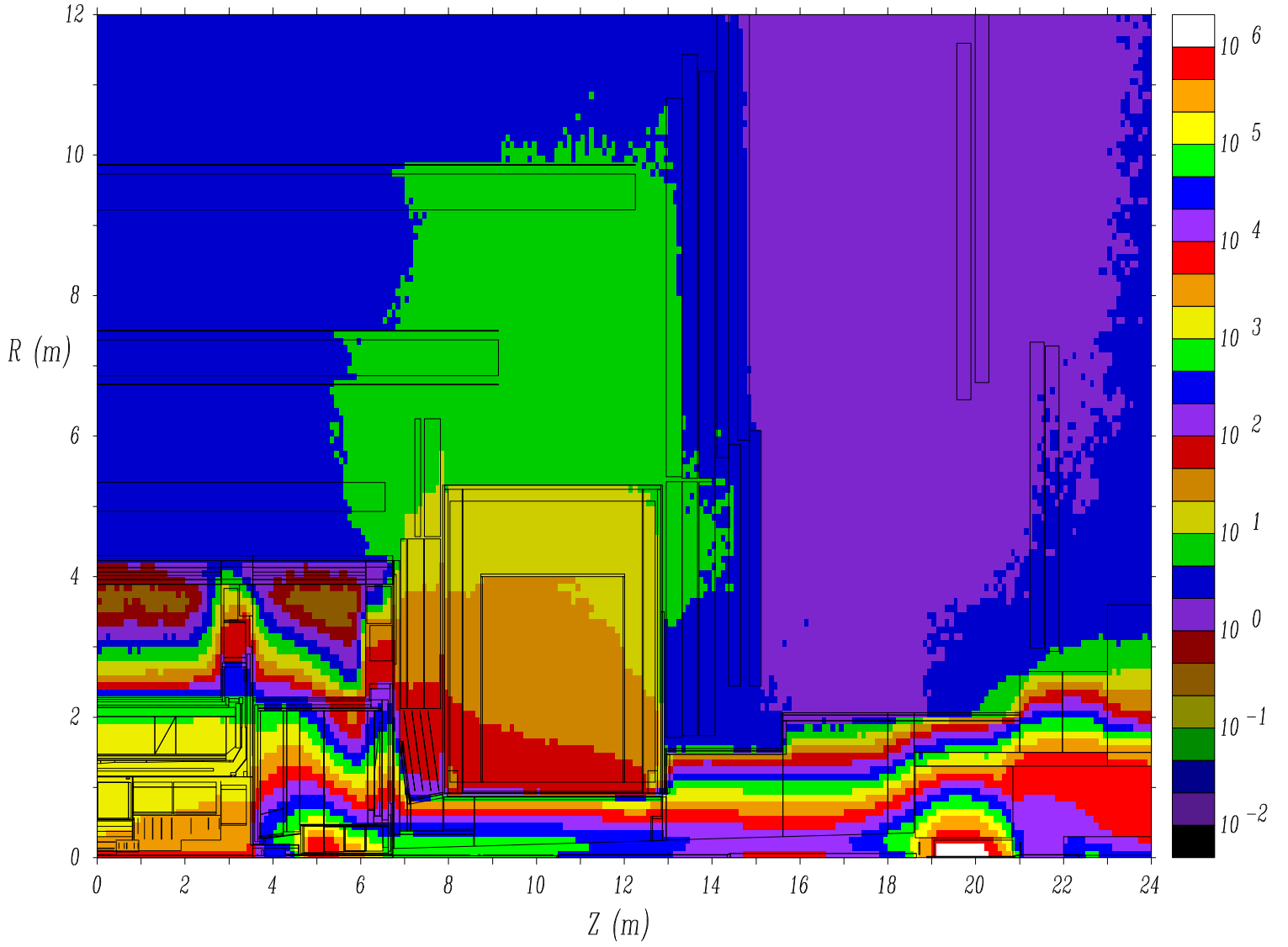
Dec01 JF0ctSameRo (5152) - Neutron Flux, KHz/cm**2
