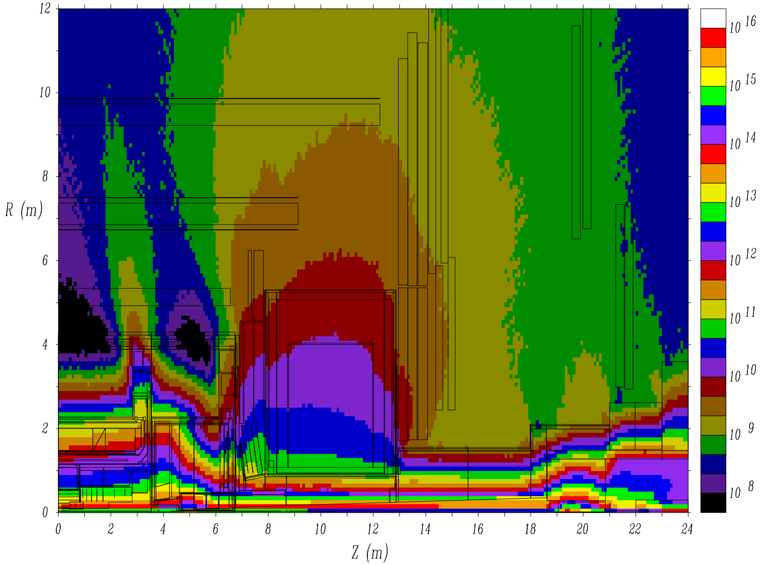
Jun02 Baseline (65180) - Hadron Flux > 20 \text{ MeV/cm}^2/\text{Yr}
