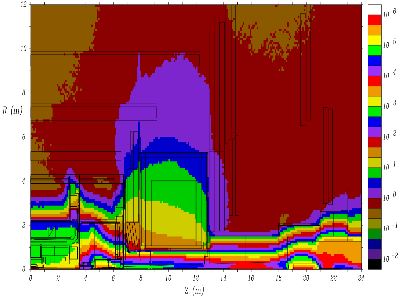
Jun02 Baseline (65180) - Neutrons > 100 keV, KHz/cm**2
