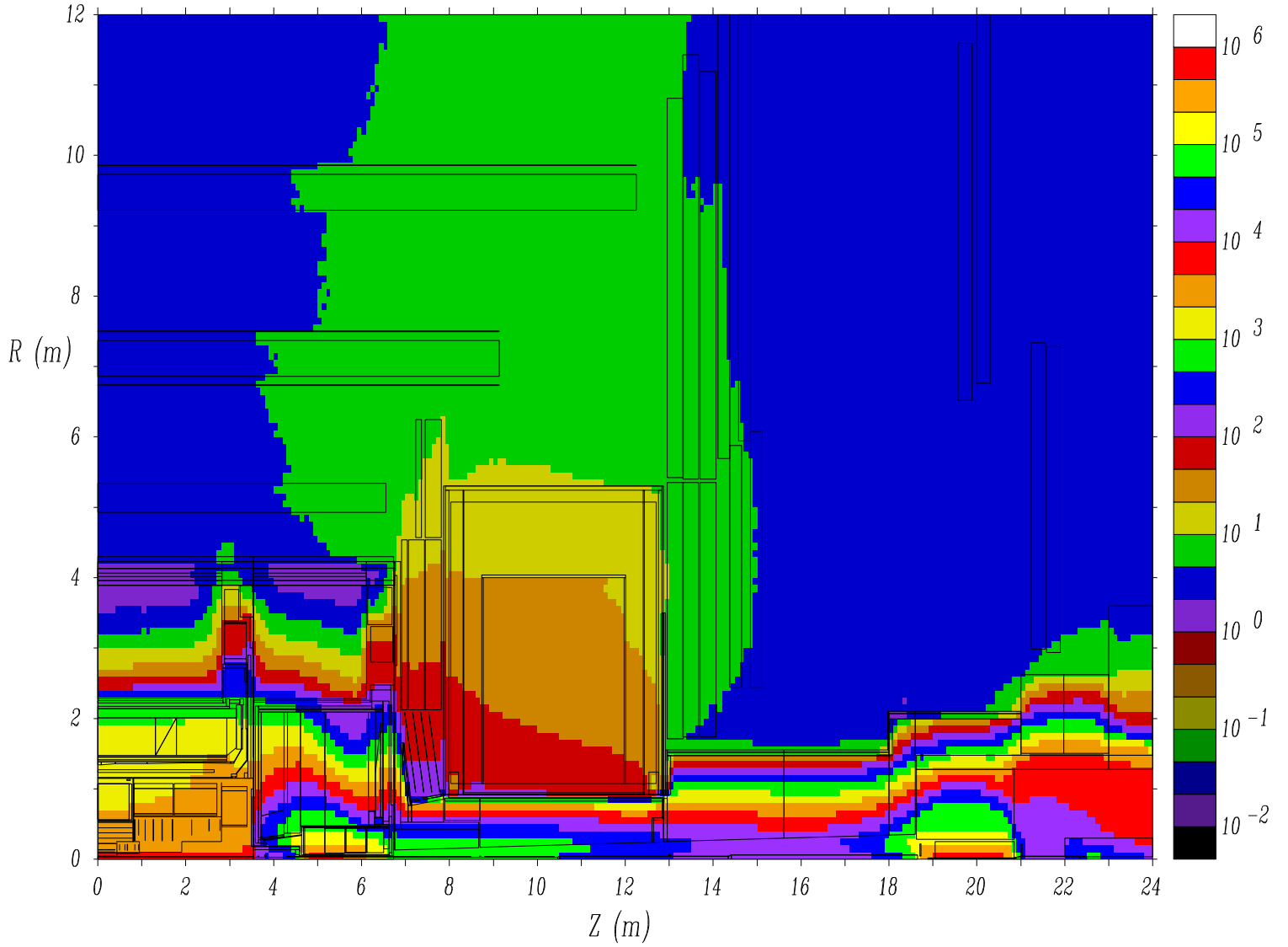
Jun02 Baseline (65180) - Neutron Flux, \text{KHz}/\text{cm}^{**2}
