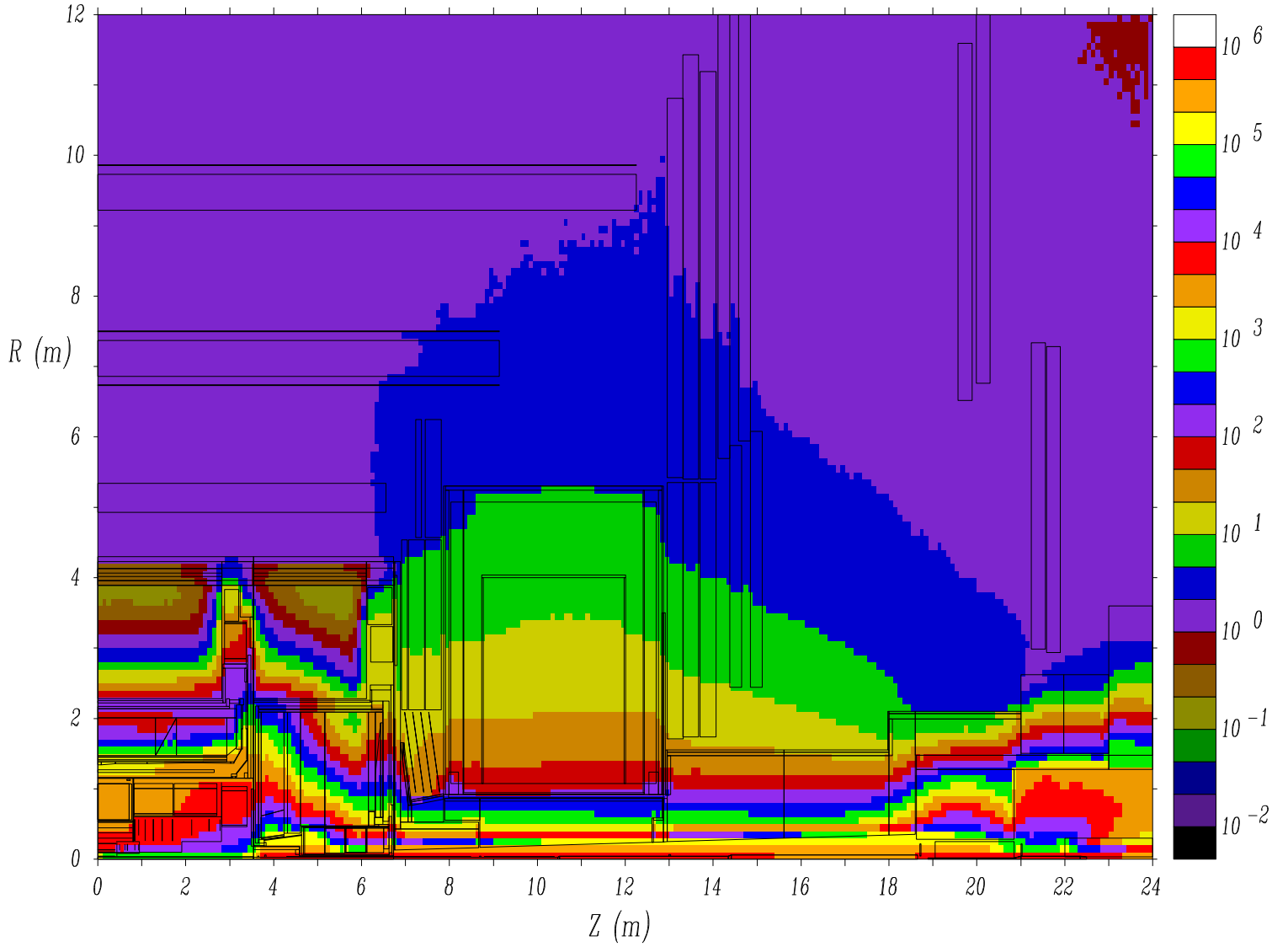
Jun02 Baseline (65180) - Photon Flux, KHz/cm**2
