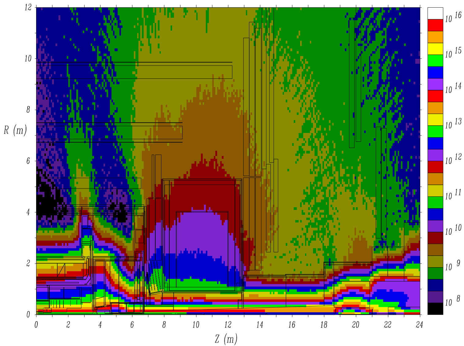
Dec01 NoOct1 SmOct2 (5958) - Hadron Flux > 20 MeV/cm**2/Yr
