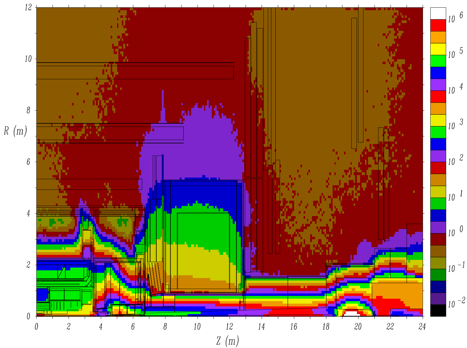
Dec01 No0ct1 Sm0ct2 (5958) - Neutrons > 100 keV, KHz/cm**2
