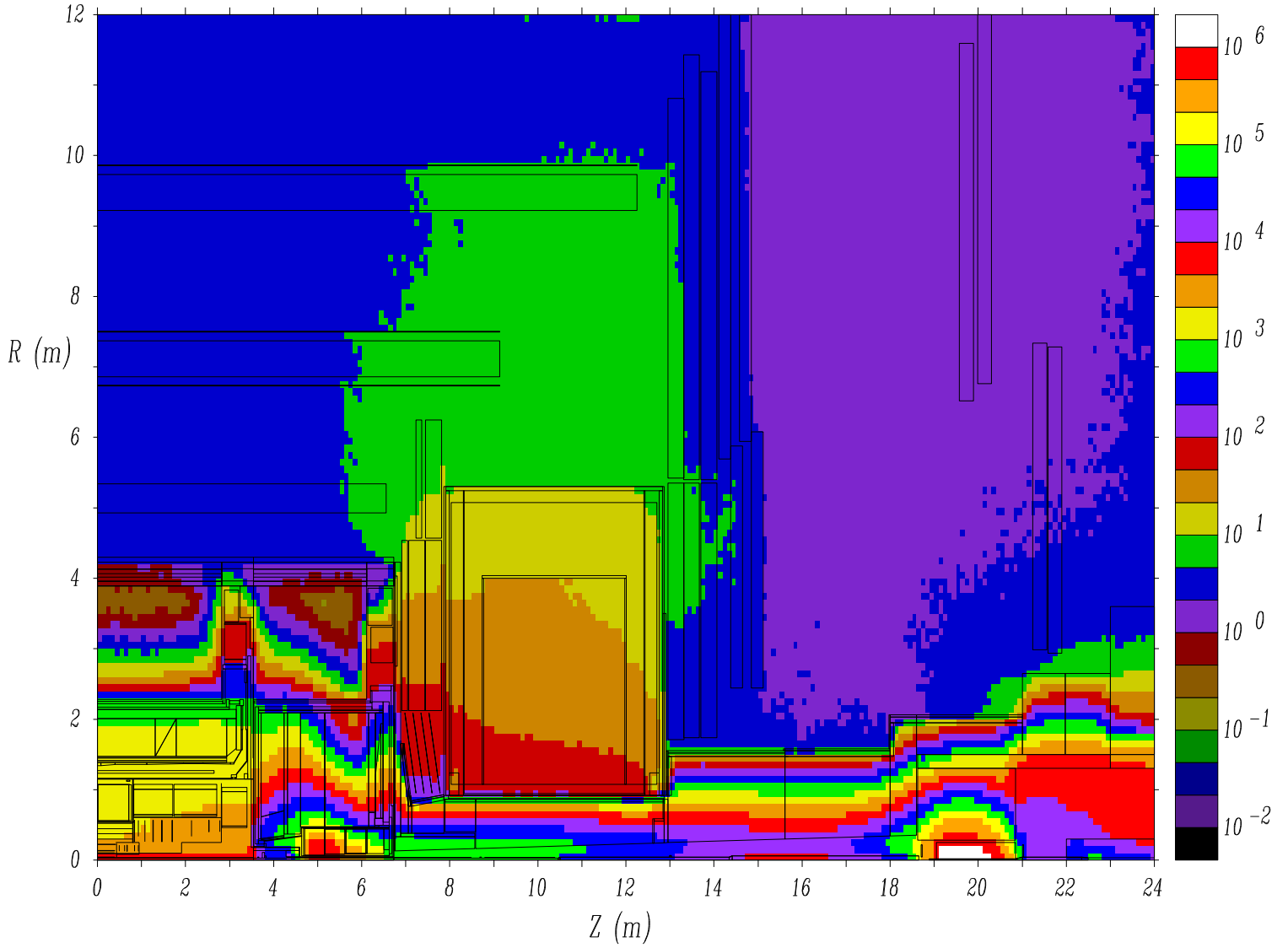
Dec01 NoOct1 SmOct2 (5958) - Neutron Flux, KHz/cm**2
